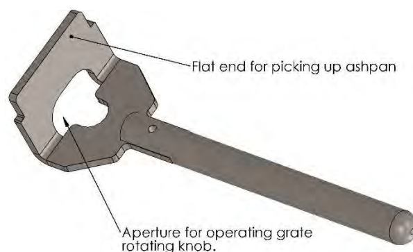
Fig 1 - Operating Tool Details
