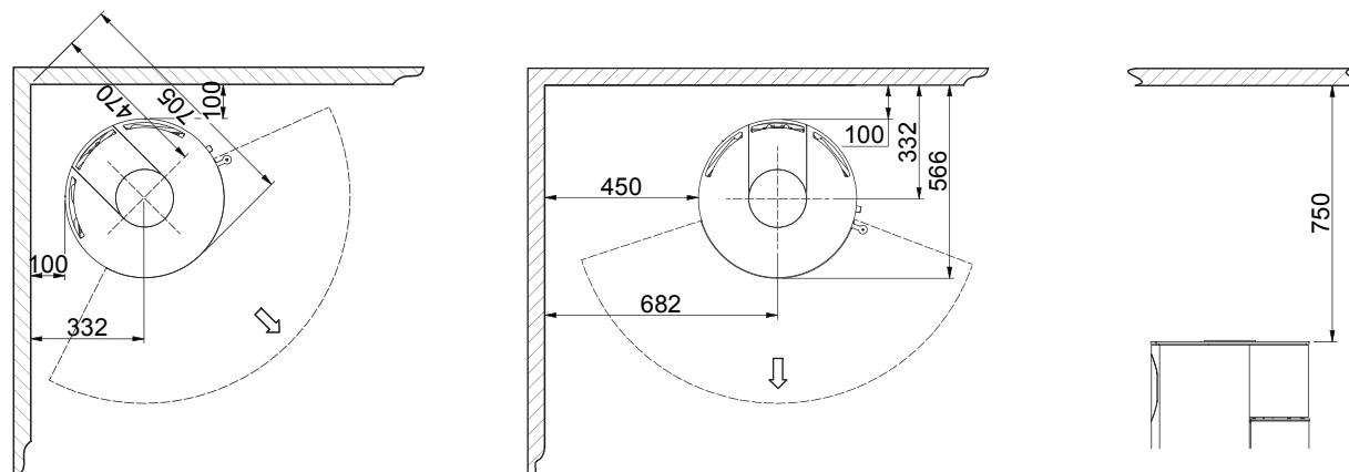
Minimum distance to flammable materials
