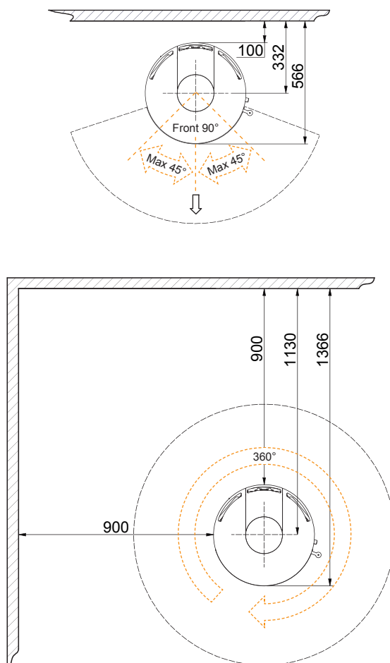
Minimum distance to flammable materials with rotating base (Accessory)
