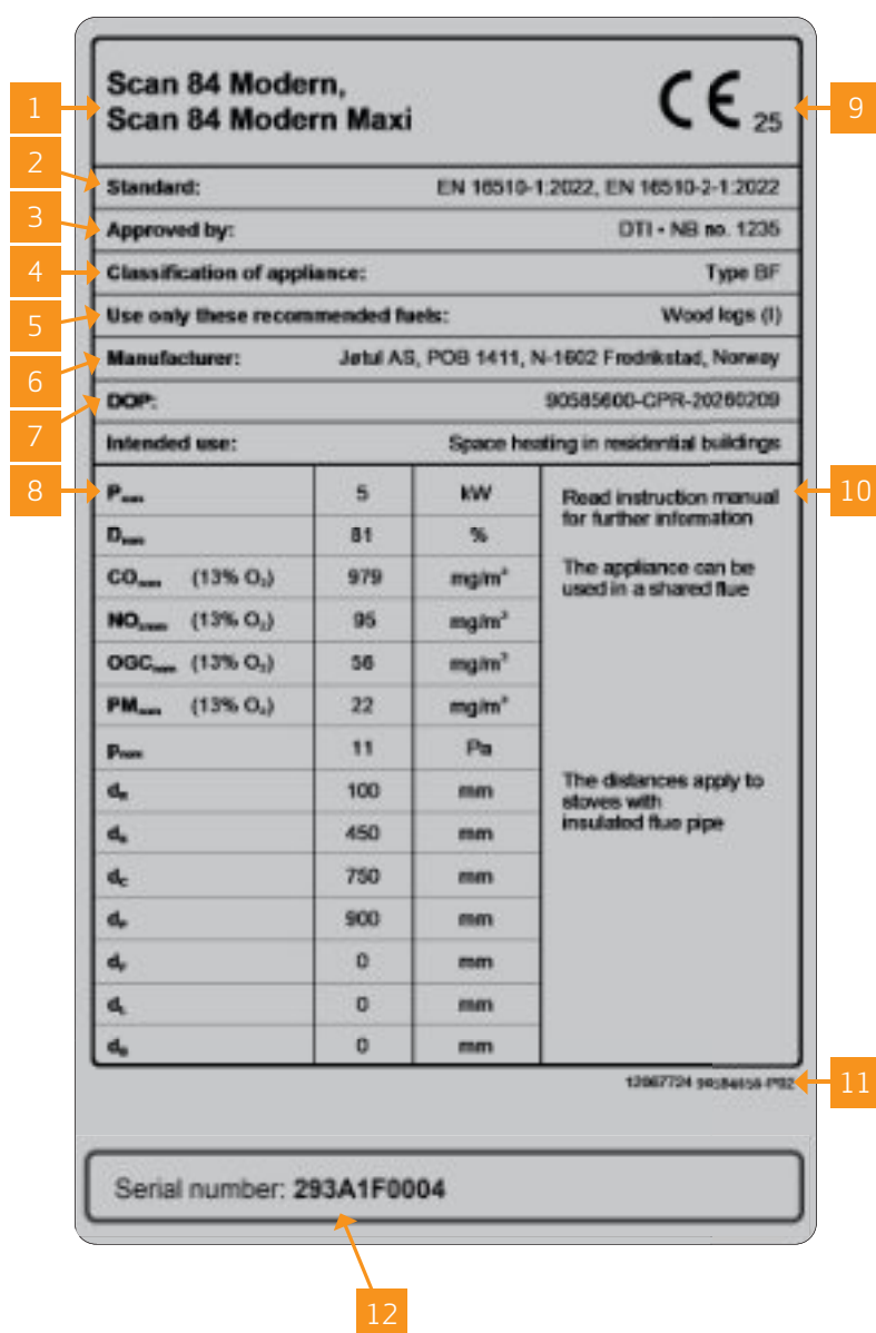
Type plate
